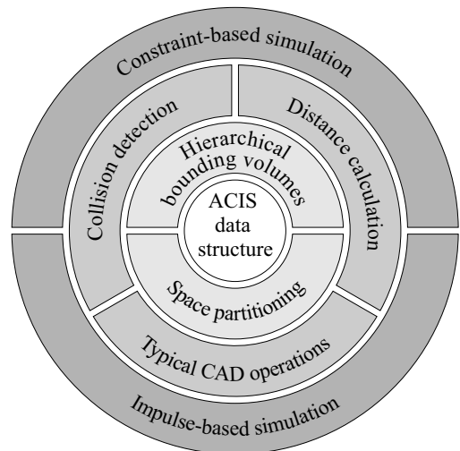
Figure 2: The structure of SiLVIA.
